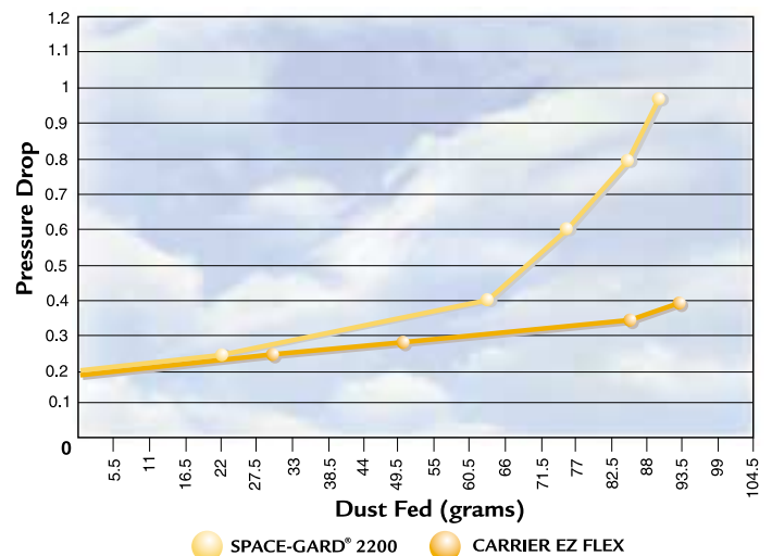
DUST FED vs. PRESSURE DROP
